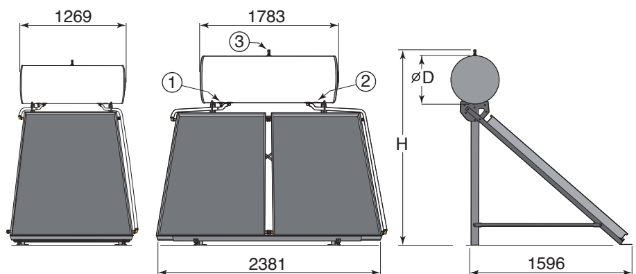
STMO 150-2 STMO 200-2
